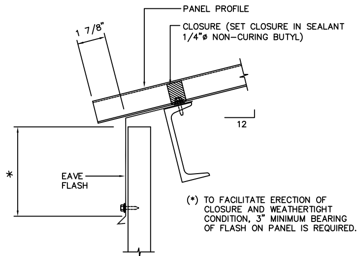
EAVE DETAIL
