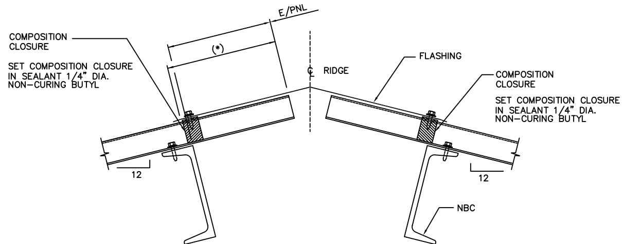
RIDGE DETAIL
